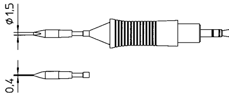
0054460599 RT5 Chisel Tip 30° bent 0.030" x 0.020" (0,8mm x 0,4mm)
